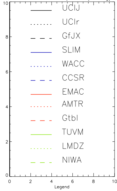
Part 1a: no aerosol/cloud (15 deg)
