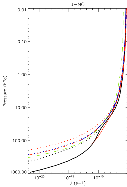
Part 1a: no aerosol/cloud (15 deg)
