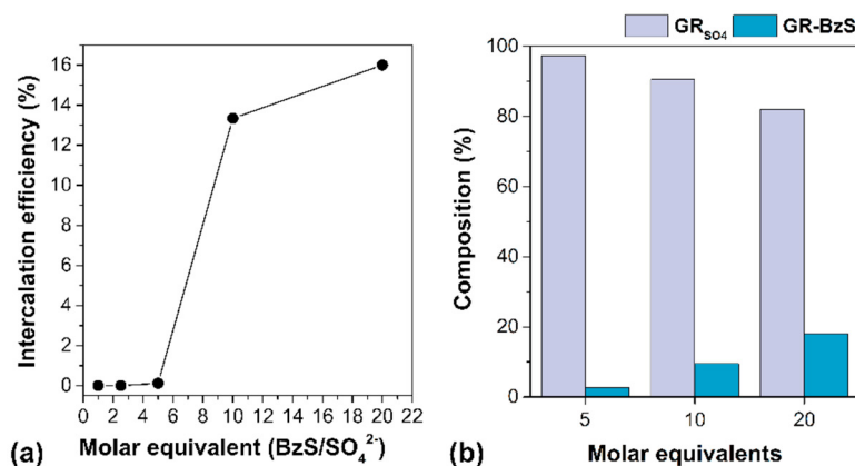
Fig. 4. (a) Intercalation efficiency of BzS calculated from the Rietveld refinement of the 001 peaks of \text{GR}_{\text{SO}_4} and GR-BzS. (b) Composition of BzS-interacted \text{GR}_{\text{SO}_4} based on the calculated areas of the 001 peaks of \text{GR}_{\text{SO}_4} and GR-BzS.
