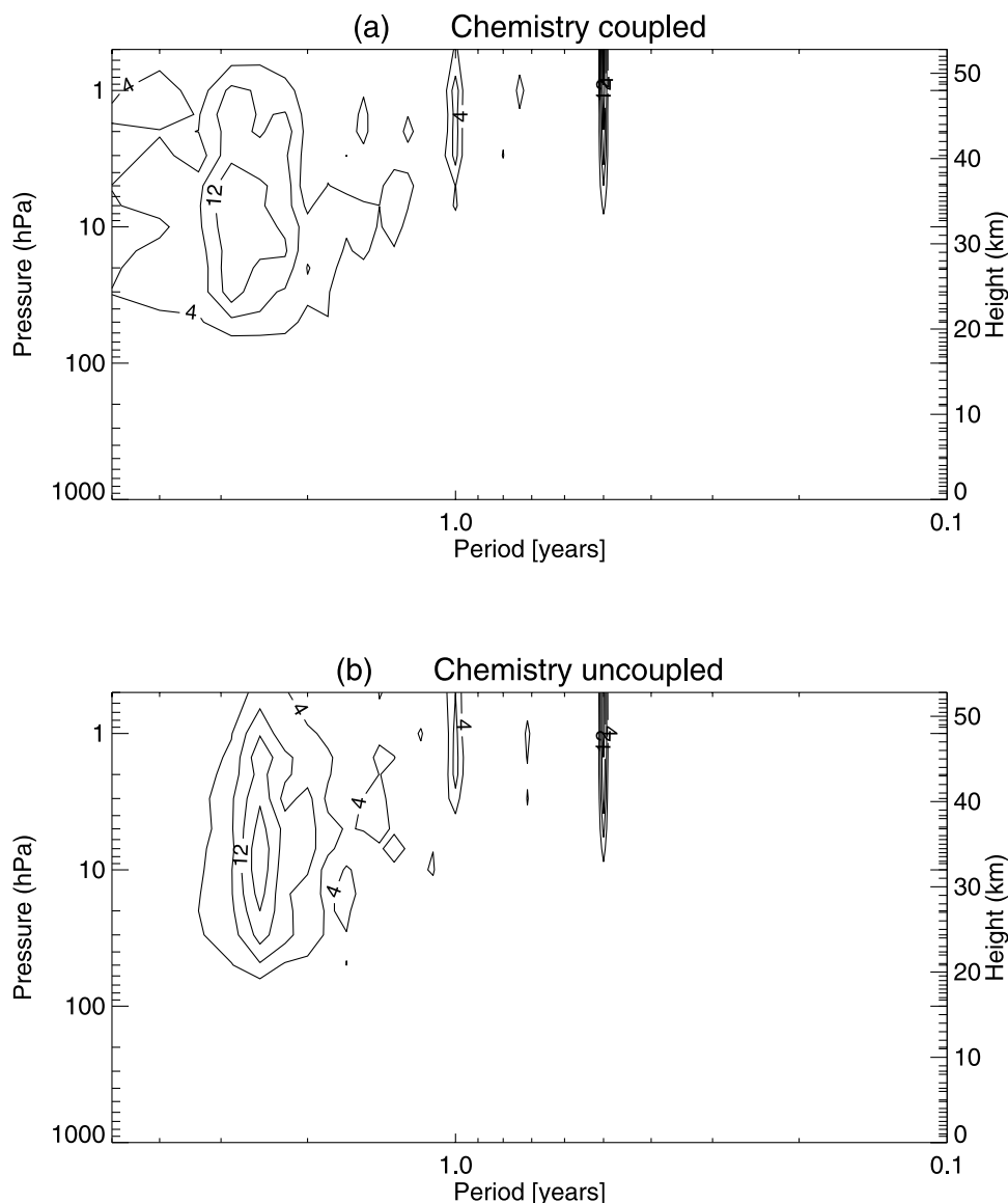
Figure 3. Fourier spectrum of the model equatorial zonal mean zonal wind for (a) the coupled run and (b) the uncoupled run. The Fourier frequency analysis was performed for each model level. The contours are drawn at the Fourier amplitudes of 1, 2, 4, 8, and 12 \text{m s}^{-1} .
