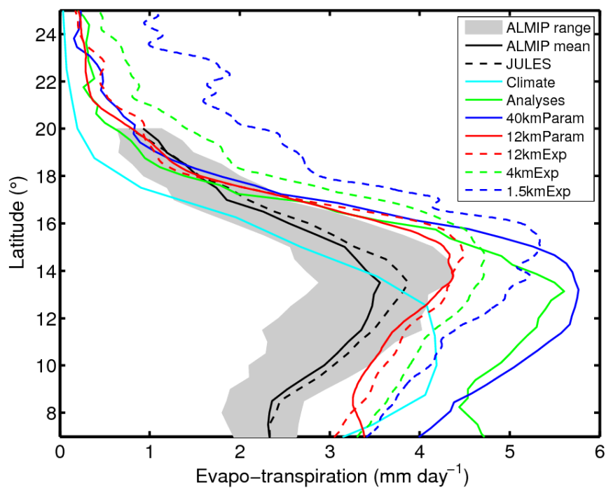
Figure 8 Mean latitude plot of evapotranspiration averaged between 8°W and 6°E. The data from 12kmParam, 12kmExp, 4kmExp and 1.5kmExp are smoothed to 40 km resolution. The grey area represents the range (minimum and maximum) of the ALMIP simulations.
