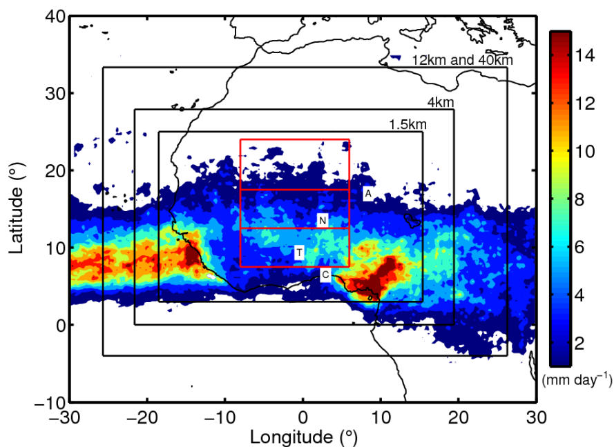
Figure 2 Mean daily TRMM rainfall 0000 UTC, 25 July 2006 to 0000 UTC 3 September 2006 (shading). The limited area model domains are marked by the black lines and the red lines mark the boundaries of the averaging boxes used in Figures 12-14: north (17.5-24°N, 8°W-6°E), mid (12.5-17.5°N, 8°W-6°E) and southern (7.5-12.5°N, 8°W-6°E). Data are averaged over all three of these boxes (7.5-24°N, 8°W-6°E) in Figure 3. The locations of four radiosonde stations are also marked: 'A' = Agadez, 'N' = Niamey, 'T' = Tamale and 'C' = Cotonou.
