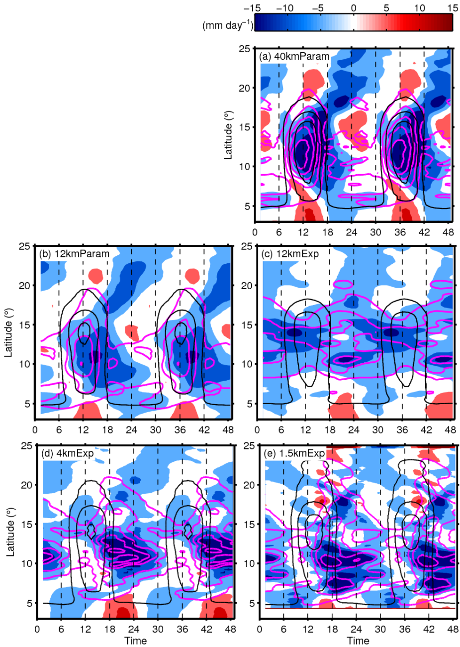
Figure 11 Mean diurnal cycle of MFD (shading), precipitation (pink contours) and evapotranspiration (black contours), averaged between -8 and 6^\circ\text{E} . The black and pink contours are at 3, 8, 13 and 18 \text{mm day}^{-1} . Red (blue) shading implies that the moisture flux is drying (wetting) the atmosphere.
