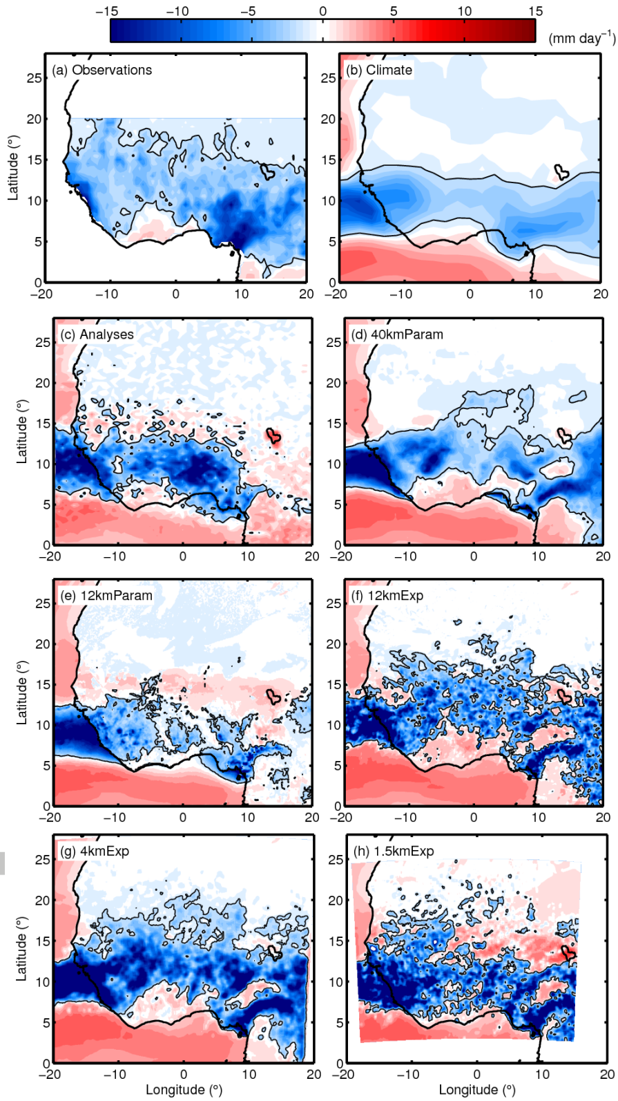
Figure 9 40-day mean E - P . The black contour is at -1 \text{ mm day}^{-1} .
