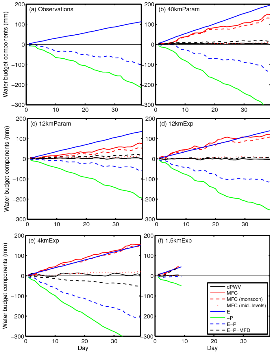
Figure 12 Cumulative plots of the terms of the water budget in the northern box (17.5-24°N). P and MFD have been multiplied by -1 so that the terms on the positive side of the y-axis add moisture to the atmosphere and the terms on the negative side of the y-axis remove moisture from the atmosphere. It follows that -1 * MFD = MFC . dPWV is the change in PWV over the 40 days.
