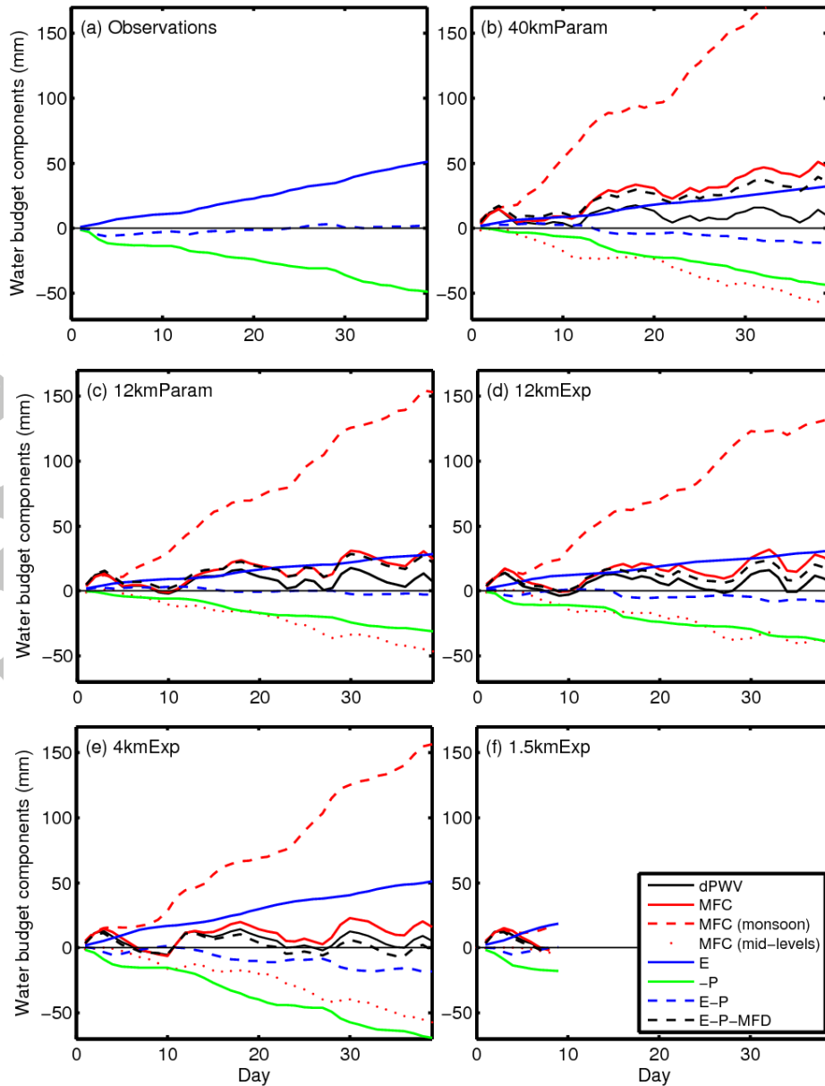
Figure 13 Cumulative plots of the terms of the water budget in the southern box (7.5-12.5N). P and MFD have been multiplied by -1 so that the terms on the positive side of the y-axis add moisture to the atmosphere and the terms on the negative side of the y-axis remove moisture from the atmosphere. It follows that -1 * MFD = MFC . dPWV is the change in PWV over the 40 days.
