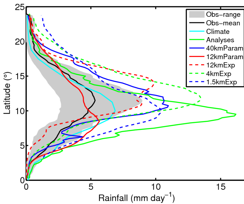
Figure 4 Mean rainfall by latitude, averaged 8°W-6°E. Data from 12kmParam, 12kmExp, 4kmExp and 1.5kmExp are smoothed to 40 km resolution. The grey area represents the range (minimum and maximum) of the satellite products.
