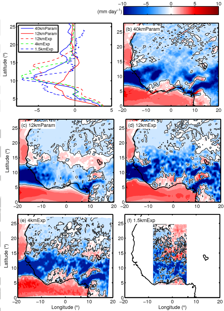
Figure 10 40-day mean MFD integrated over whole atmospheric column. (a) is averaged between 8°W and 6°E and the x-axis is MFD (mm day -1 ). The black contour is at -1 mm day -1 . Due to computational limitations MFD was only computed for 1.5kmExp within the analyses boxes marked in Figure 1 (7.5-24°N, 8°W-6°E).
