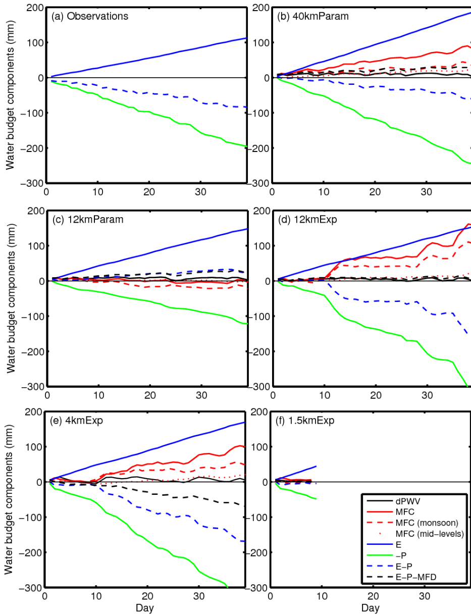
Figure 14 Cumulative plots of the terms of the water budget in the mid box (12.5-17.5°N). P and MFD have been multiplied by -1 so that the terms on the positive side of the y-axis add moisture to the atmosphere and the terms on the negative side of the y-axis remove moisture from the atmosphere. It follows that -1 \cdot \text{MFD} = \text{MFC} . dPWV is the change in PWV over the 40 days.
