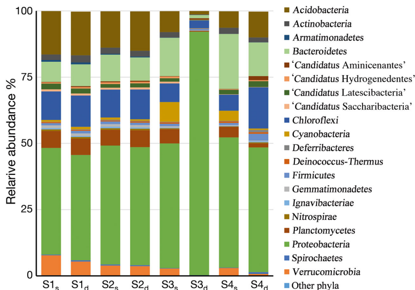
Fig. 3. Taxonomical composition of the bacterial community at the phylum level. Phyla with relative abundance below 0.1% are grouped as 'Other phyla'. Sampling sites (see Fig. 2) were S1: Boothferry, S2: Blacktoft, S3: Paull and S4: Skeffling; 's' and 'd' refer to surface and subsurface sediments, respectively
