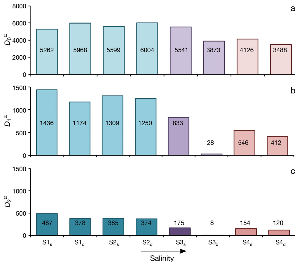
Fig. 4. Alpha-diversity ( D_q^\alpha ) at each location measured with Hill numbers ( D_q ) of different order ( q = 0, 1 and 2 ) which represent: (a) operational taxonomic unit (OTU) richness ( D_0^\alpha ), (b) common OTUs ( D_1^\alpha ) and (c) dominant OTUs ( D_2^\alpha ). The colours of the bars follow the colour code for the inner (blue), mid- (purple) and outer (pink) estuary defined by salinity variation range (colour darkens as q increases from D_0^\alpha to D_2^\alpha ). Sampling sites (see Fig. 2) were S1: Boothferry, S2: Blacktoft, S3: Paull and S4: Skeffling; 's' and 'd' refer to surface and subsurface sediments, respectively. For more details, see the 'Materials and methods'
