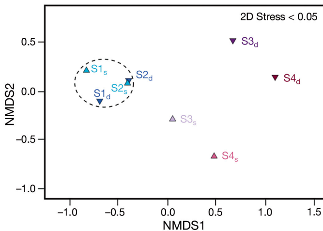
Fig. 5. Non-metric multidimensional scaling (NMDS) ordination for dissimilarities in the bacterial community distribution among samples based on Bray-Curtis distances. Samples are colour-coded according to the salinity variation zones (blue: inner, purple: mid-, pink: outer estuary). Lighter (darker) colours represent surface (subsurface) sediment samples. The dashed ellipse has been added to indicate the inner estuary samples. Sampling sites (see Fig. 2) were S1: Boothferry, S2: Blacktoft, S3: Paull and S4: Skeffling; 's' and 'd' refer to surface and subsurface sediments, respectively
