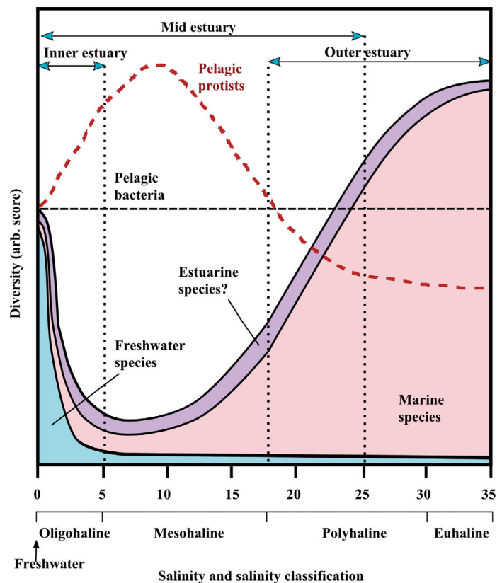
Fig. 1. Diversity variation patterns along a salinity gradient. Coloured areas represent Remane's (1934) conceptual model for the variation in macrobenthic biodiversity (after Whitfield et al. 2012, Skarlato & Telesh 2017). Variations in the diversity of pelagic protists (Telesh et al. 2011) and planktonic bacteria (Herlemann et al. 2011) are shown as dashed lines (red and black, respectively). The dotted lines indicate boundaries for the salinity zonation defined for the Humber estuary (see 'Materials and methods')
