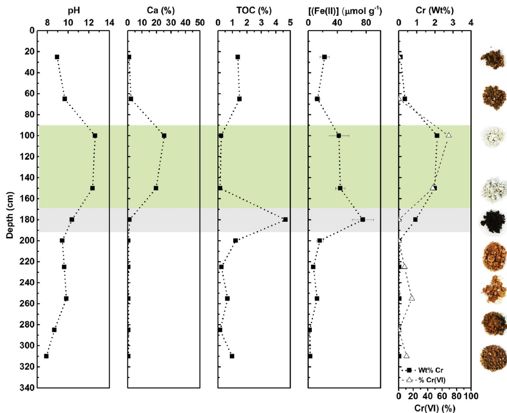
Fig. 2. Geochemical (and colour) variation in solid samples recovered from BH2. COPR waste and black organic-rich clay horizons marked by green and grey bands respectively. (For interpretation of the references to colour in this figure legend, the reader is referred to the web version of this article.)
