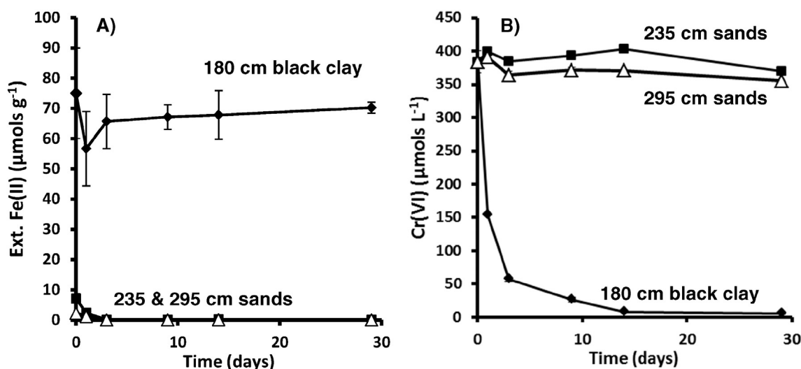
Fig. 5. Results from microcosm tests using sediments recovered from below the COPR waste in BH2 mixed with Cr(VI)-containing site leachate. A) Variation in 0.5 N HCl extractable Fe(II) and, B) variation in aqueous Cr(VI) concentrations. Error bars are 1 \sigma of triplicate microcosms and were not shown are less than the size of the symbol used.
