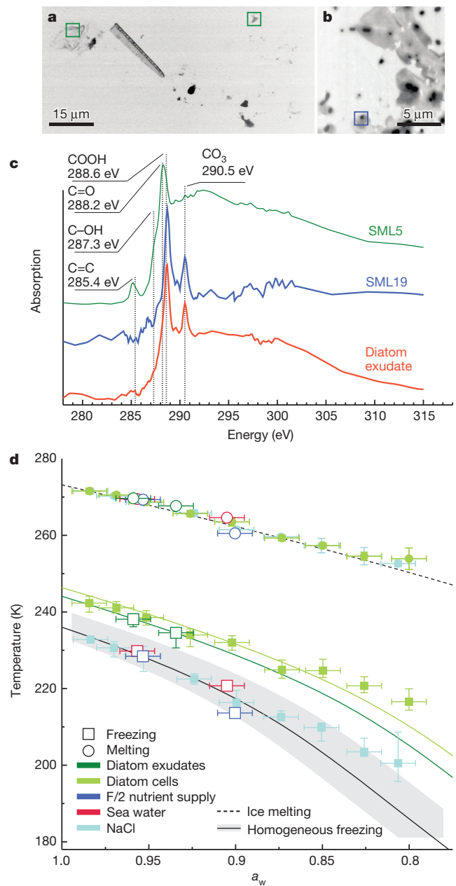
Figure 3 | Spectroscopic analysis of Arctic SML samples and freezing experiments with diatom exudate. a, b , X-ray images of Arctic SML5 ( a ) and SML19 ( b ). Example locations at which spectra were acquired are indicated by green and blue boxes. c , X-ray absorption spectra of organic material in SML5, SML19 and exudates from the diatom T. pseudonana . d , Freezing and melting temperatures, collected using the water-activity-controlled immersion freezing experiment (WACIFE), as a function of water activity ( a_w ) for nanolitre volume droplets containing T. pseudonana exudates, and filtered and autoclaved natural sea water with and without f/2 nutrients. Heterogeneous ice nucleation temperatures in the presence of diatom cells and homogeneous ice nucleation of aqueous NaCl droplets are shown for comparison 6,32 . Vertical error bars represent 10th and 90th percentiles of about 300 individual freezing events. Horizontal error bars indicate the uncertainty in a_w of \pm 0.01 .
