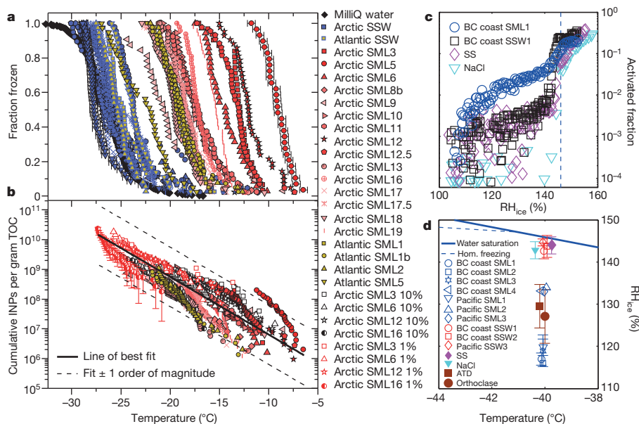
Figure 2 | Ice nucleation by material in the SML. a , Immersion mode fraction frozen curves for 1 \mu\text{l} Arctic and Atlantic SML and SSW droplets determined using the microlitre nucleation by immersed particle instrument ( \mu\text{l} -NIPI), with example temperature uncertainties included. b , The cumulative number of INPs per gram of total organic carbon (TOC). Selected samples were diluted with ultra-pure (MilliQ) water to 10% and 1% of initial concentration. Uncertainties are included where error bars are larger than data points (see Methods for details). Equation for fit to data is \text{INPs per gram TOC} = \exp[11.2186 - (0.4459 \times T)] ; note that temperature, T , is in ^\circ\text{C} . c , Ice nucleation by British Columbia (BC) coast
